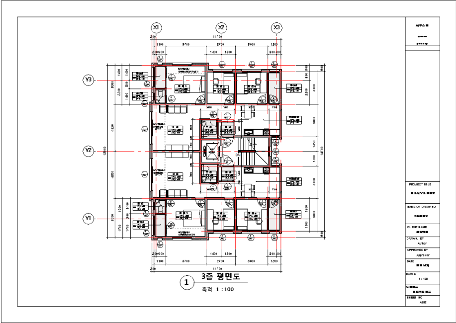
[평면도]
