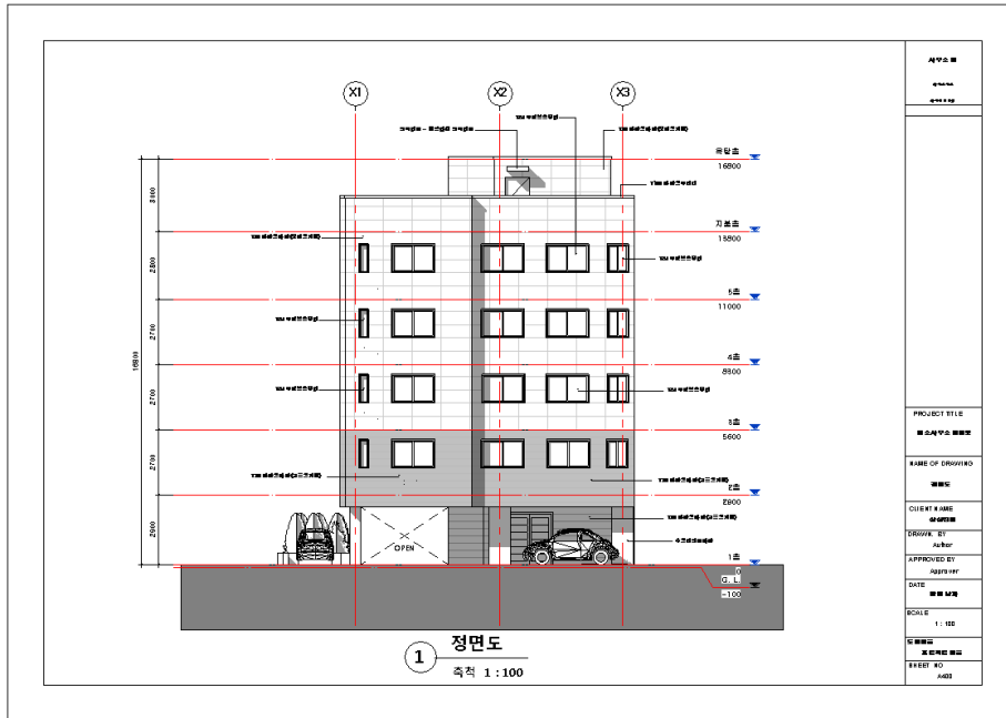
[입면도]
