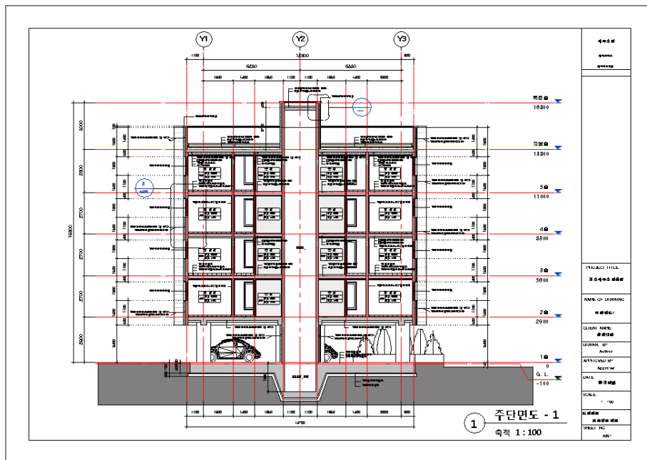
[단면도]
